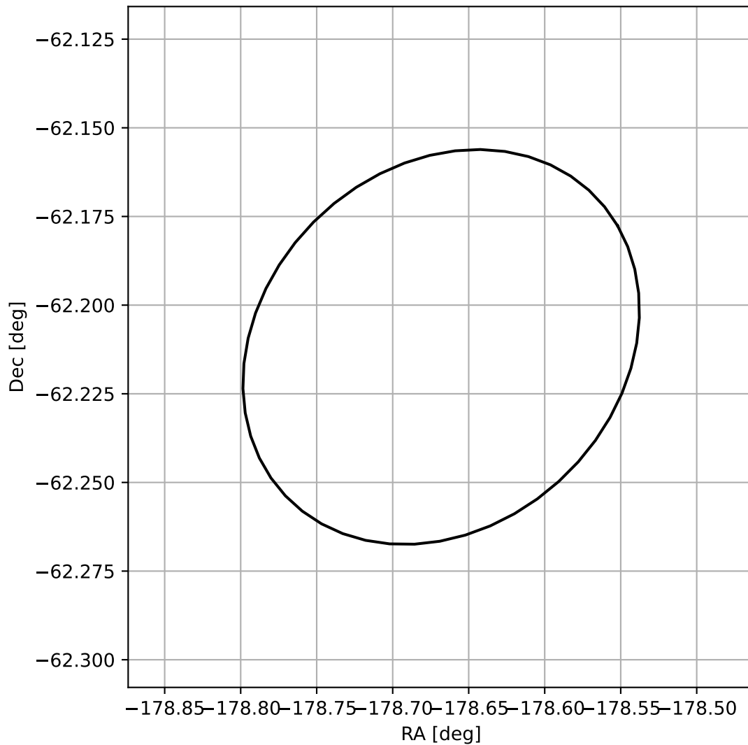
4FGL J1205.3-6212
