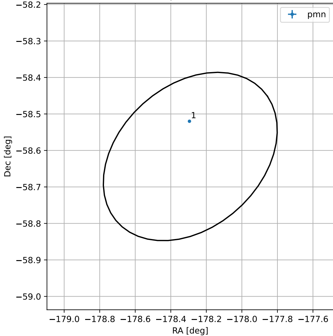
4FGL J1206.8-5836
