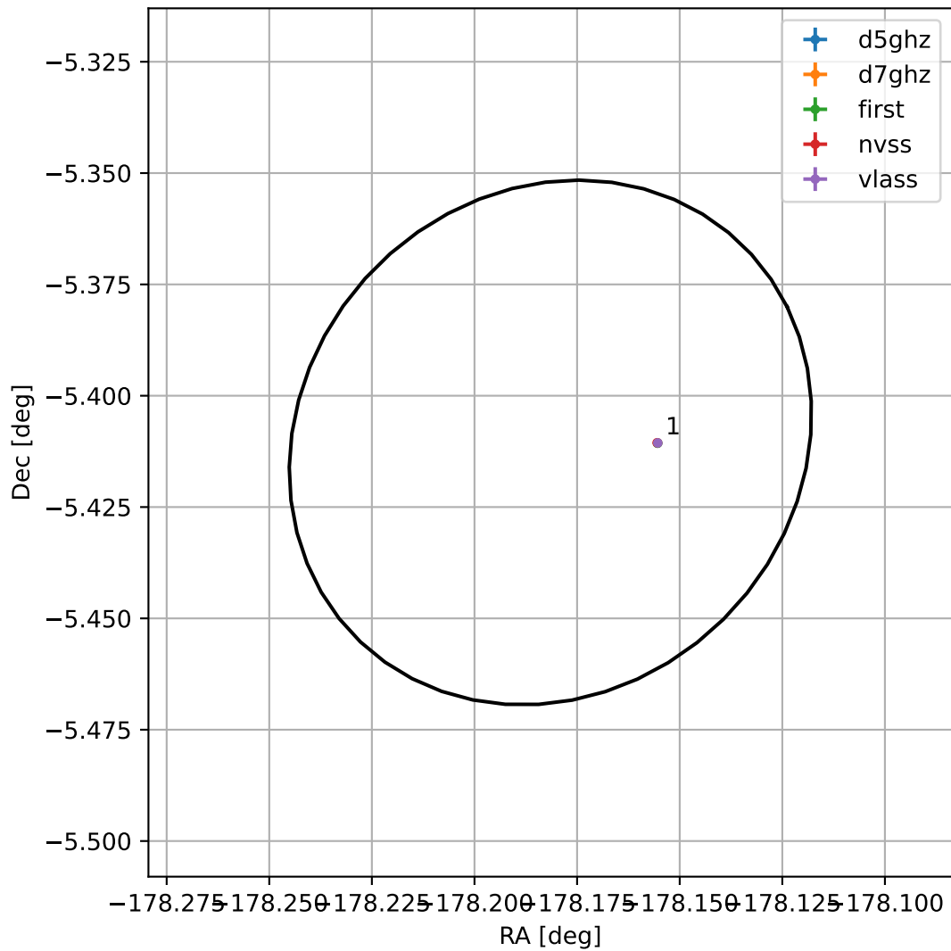
4FGL J1207.2-0524
