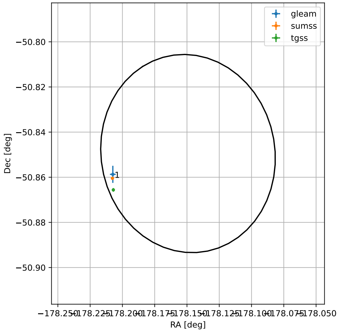
4FGL J1207.4-5050
