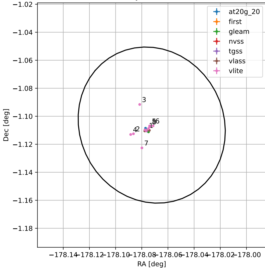
4FGL J1207.7-0106
