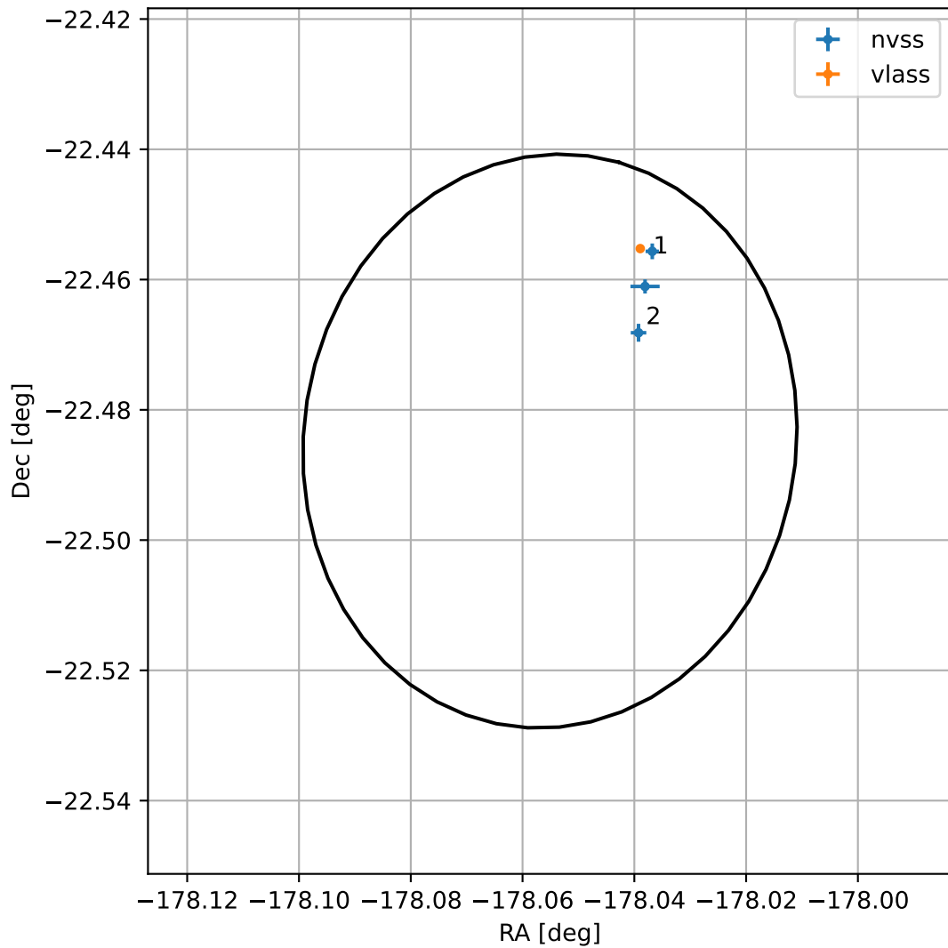
4FGL J1207.7-2229
