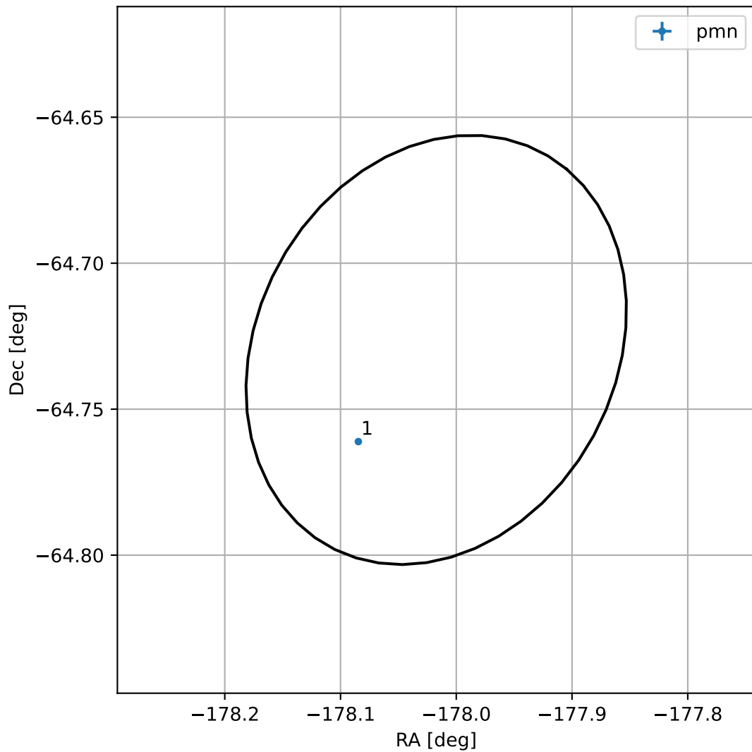
4FGL J1207.9-6443
