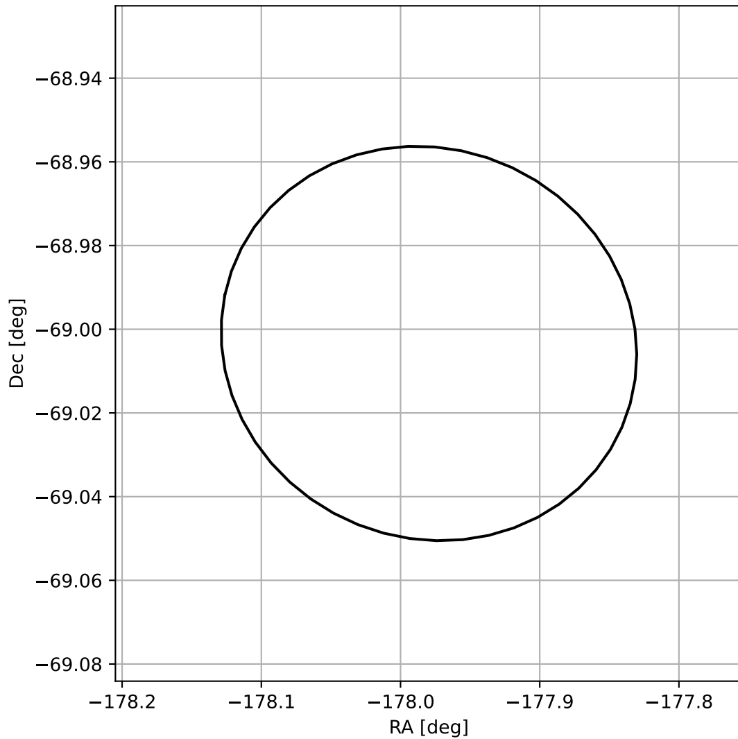
4FGL J1208.0-6900
