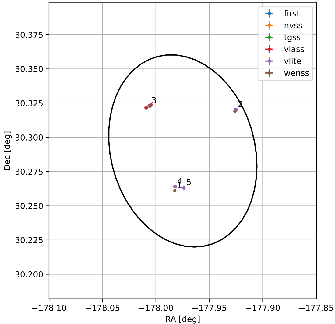
4FGL J1208.1+3017
