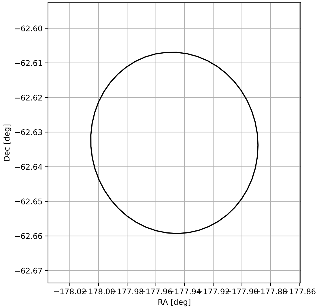
4FGL J1208.2-6237
