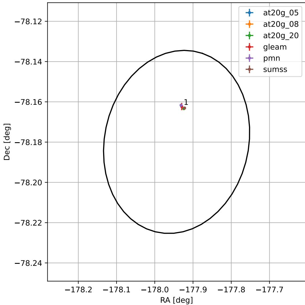
4FGL J1208.2-7810
