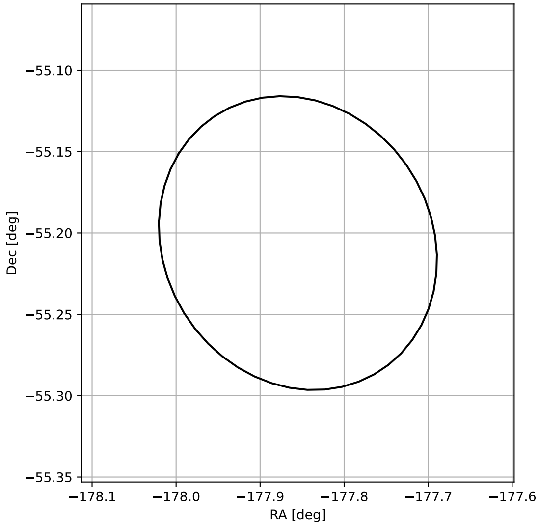
4FGL J1208.5-5512
