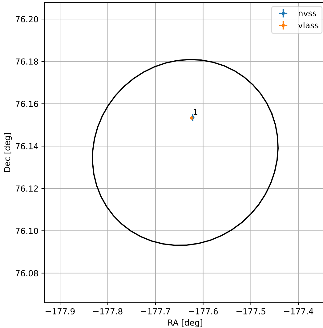
4FGL J1209.4+7608
