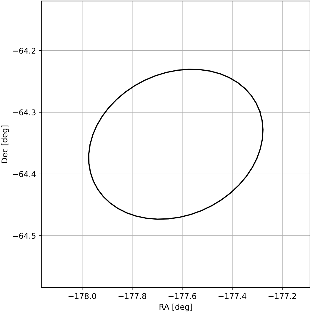
4FGL J1209.4-6421
