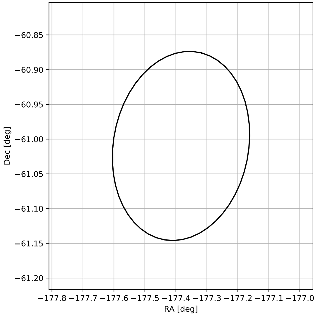
4FGL J1210.4-6100
