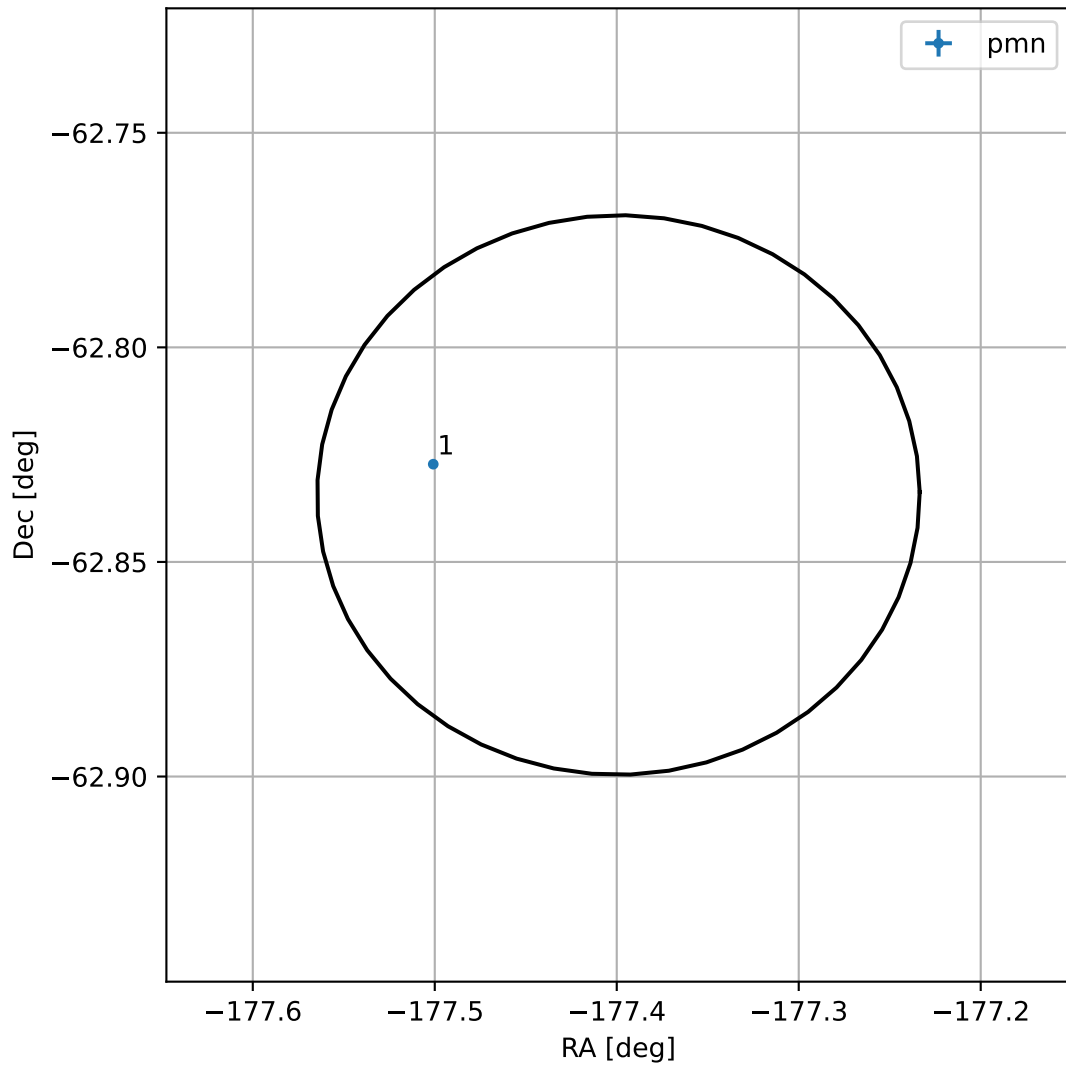
4FGL J1210.4-6250
