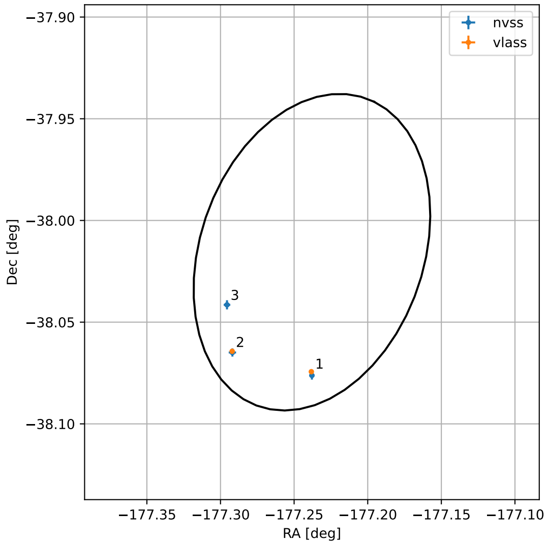
4FGL J1211.0-3800
