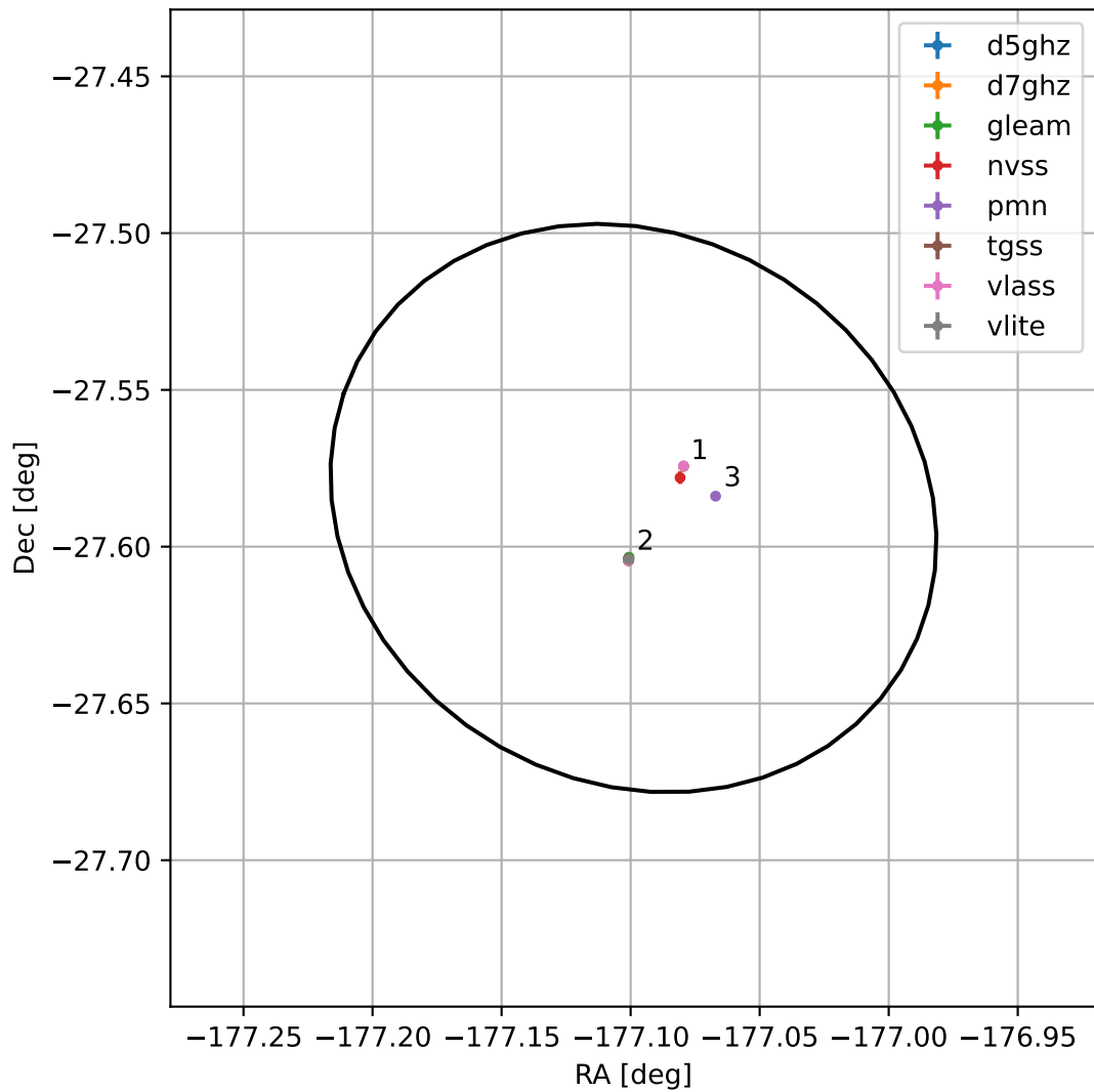
4FGL J1211.6-2735
