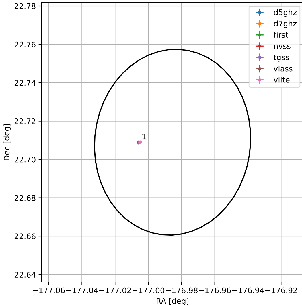
4FGL J1212.0+2242
