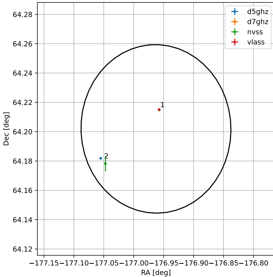
4FGL J1212.1+6412
