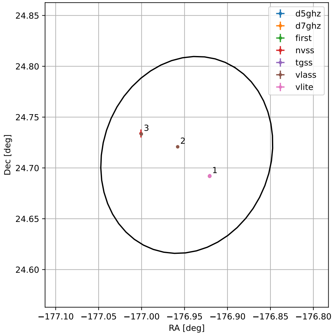
4FGL J1212.2+2442
