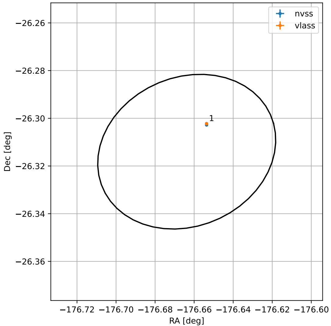
4FGL J1213.3-2618
