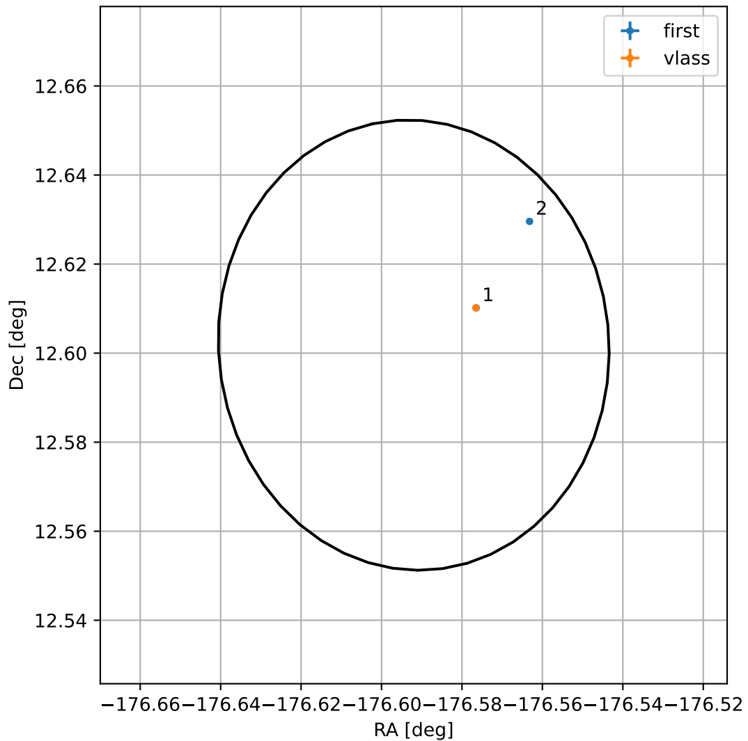
4FGL J1213.6+1236
