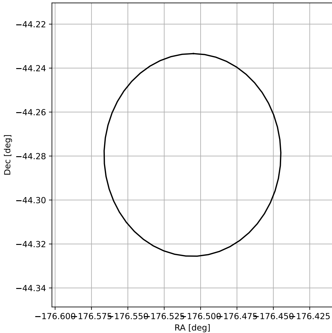
4FGL J1213.9-4416
