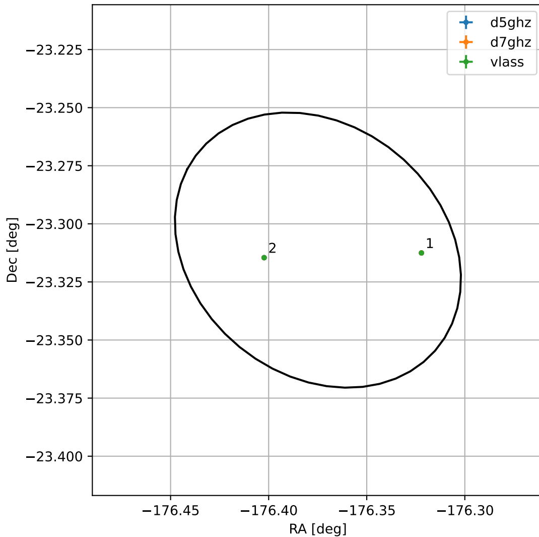
4FGL J1214.5-2318
