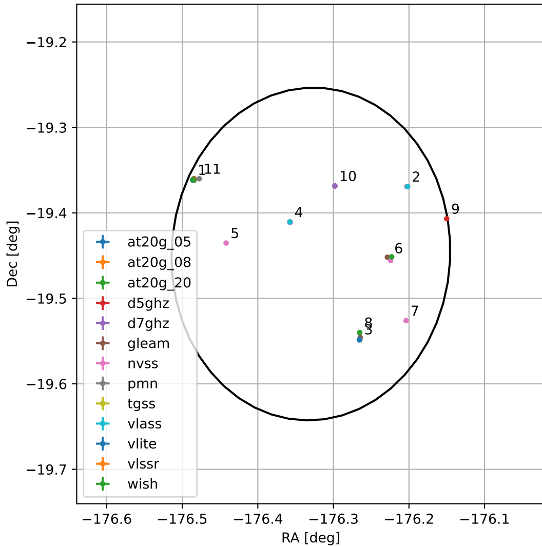
4FGL J1214.6-1926
