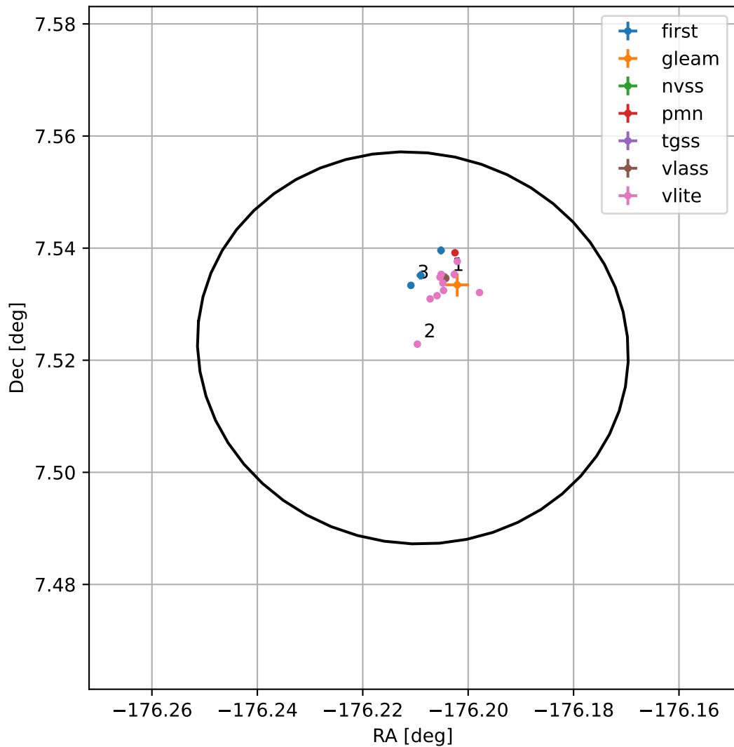
4FGL J1215.1+0731
