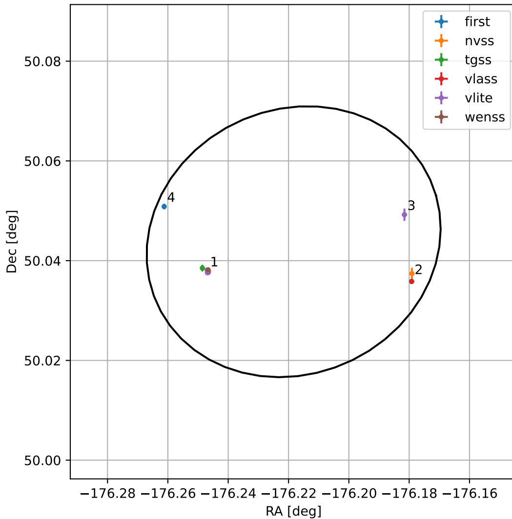
4FGL J1215.1+5002
