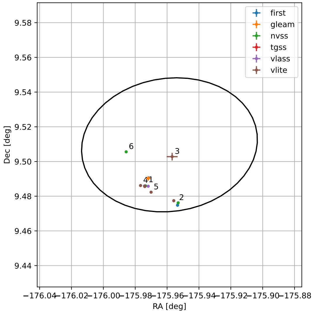
4FGL J1216.1+0930
