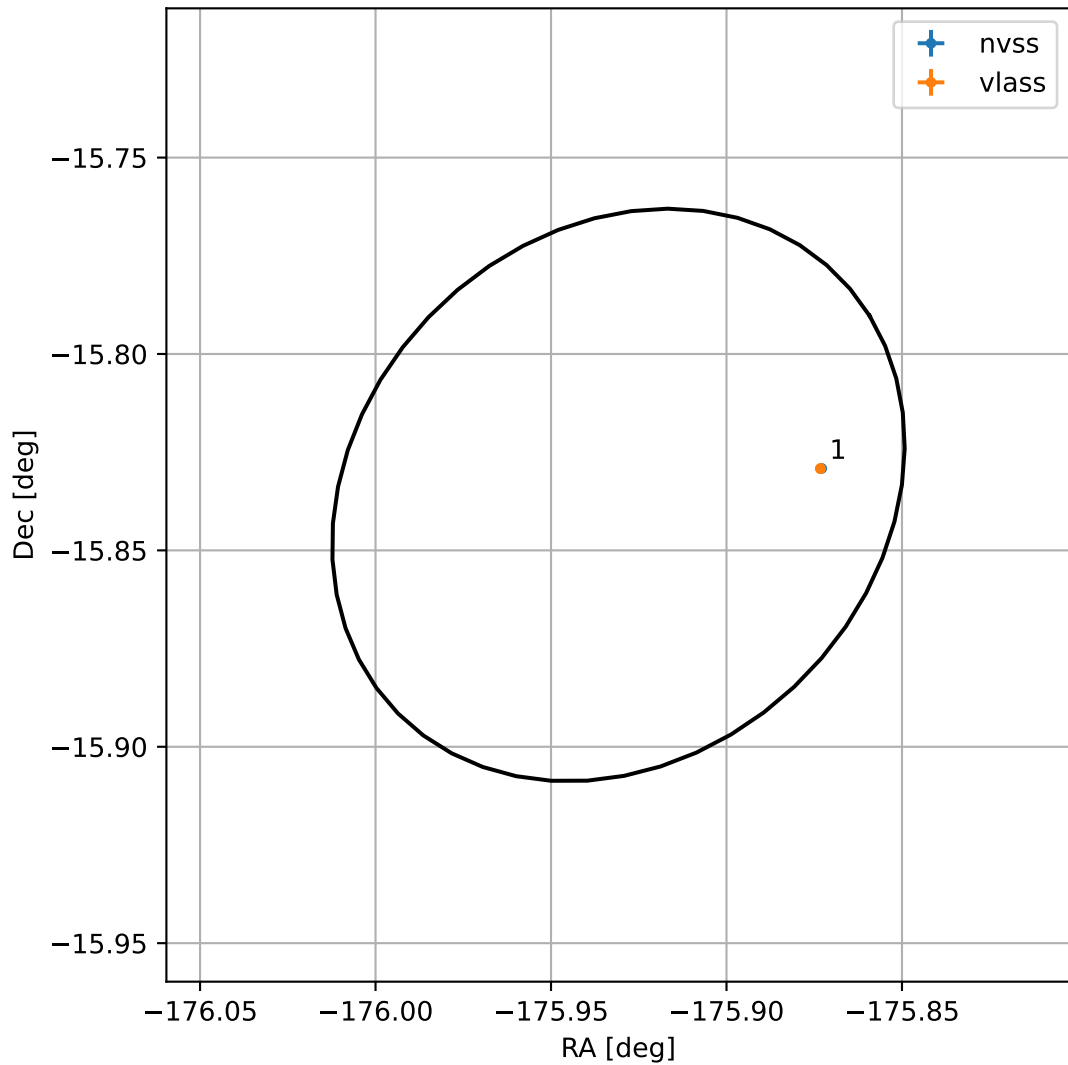
4FGL J1216.2-1550
