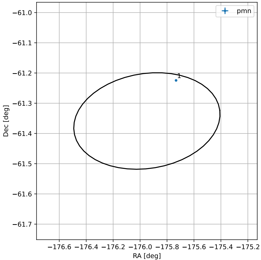
4FGL J1216.2-6121
