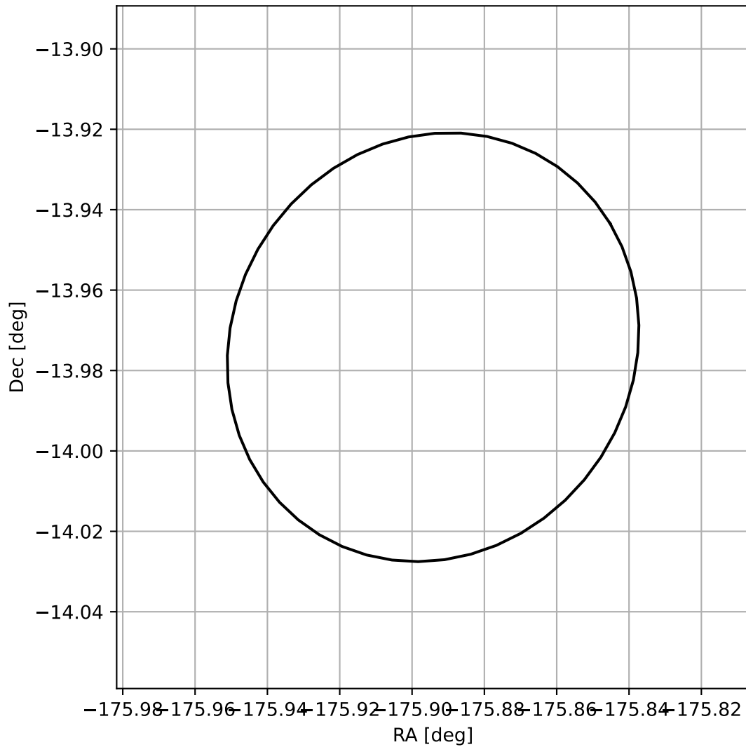
4FGL J1216.4-1358
