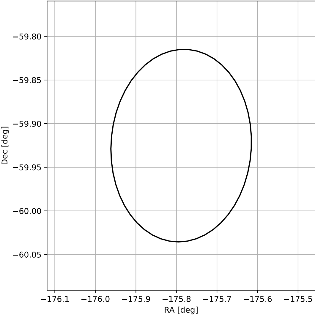
4FGL J1216.8-5955
