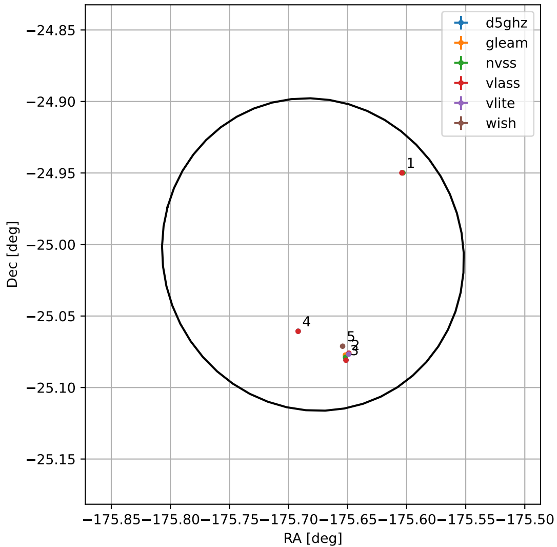
4FGL J1217.2-2500
