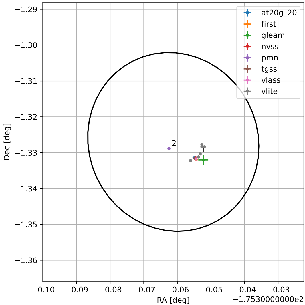
4FGL J1218.5-0119
