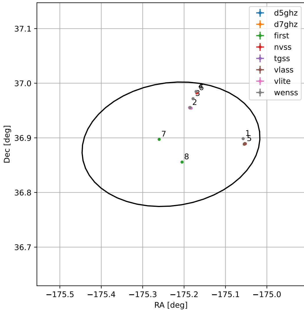
4FGL J1219.0+3653
