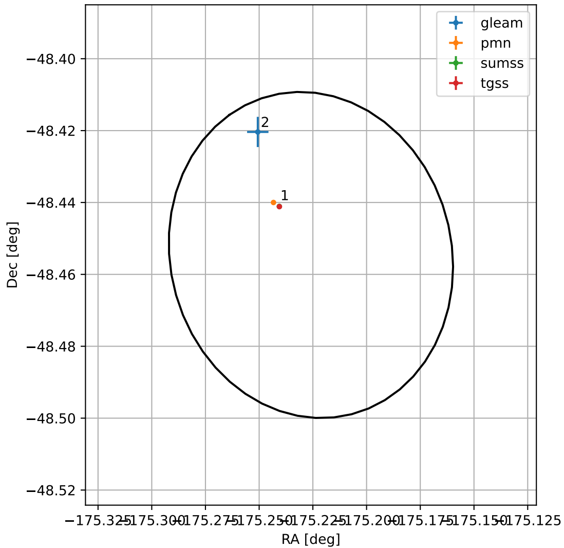
4FGL J1219.0-4827
