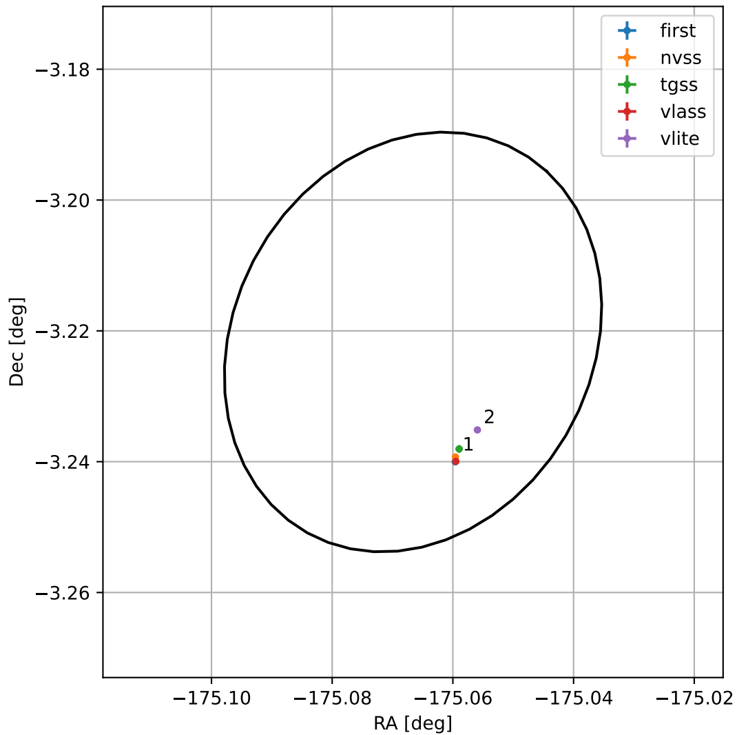
4FGL J1219.7-0313
