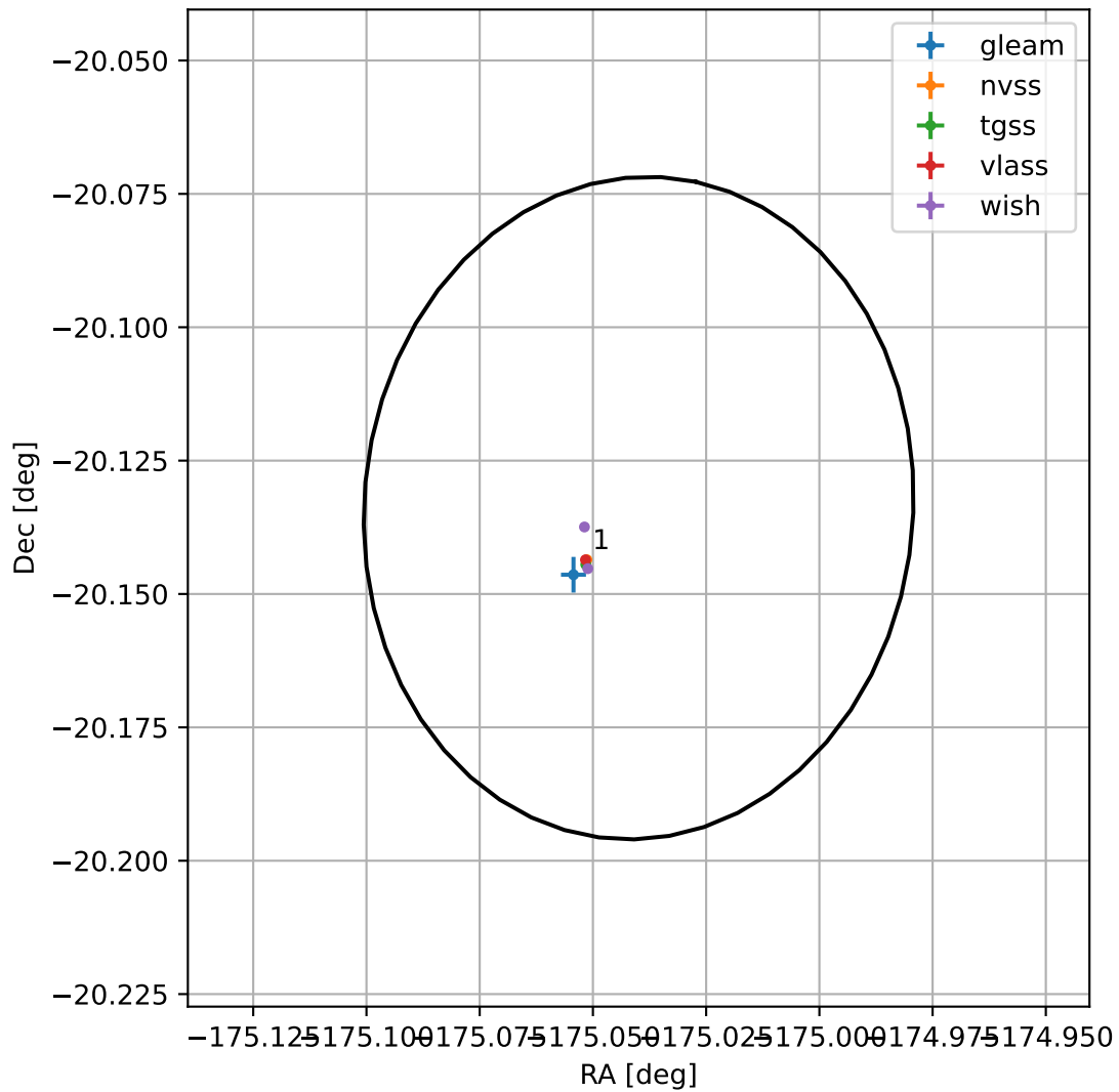
4FGL J1219.8-2008
