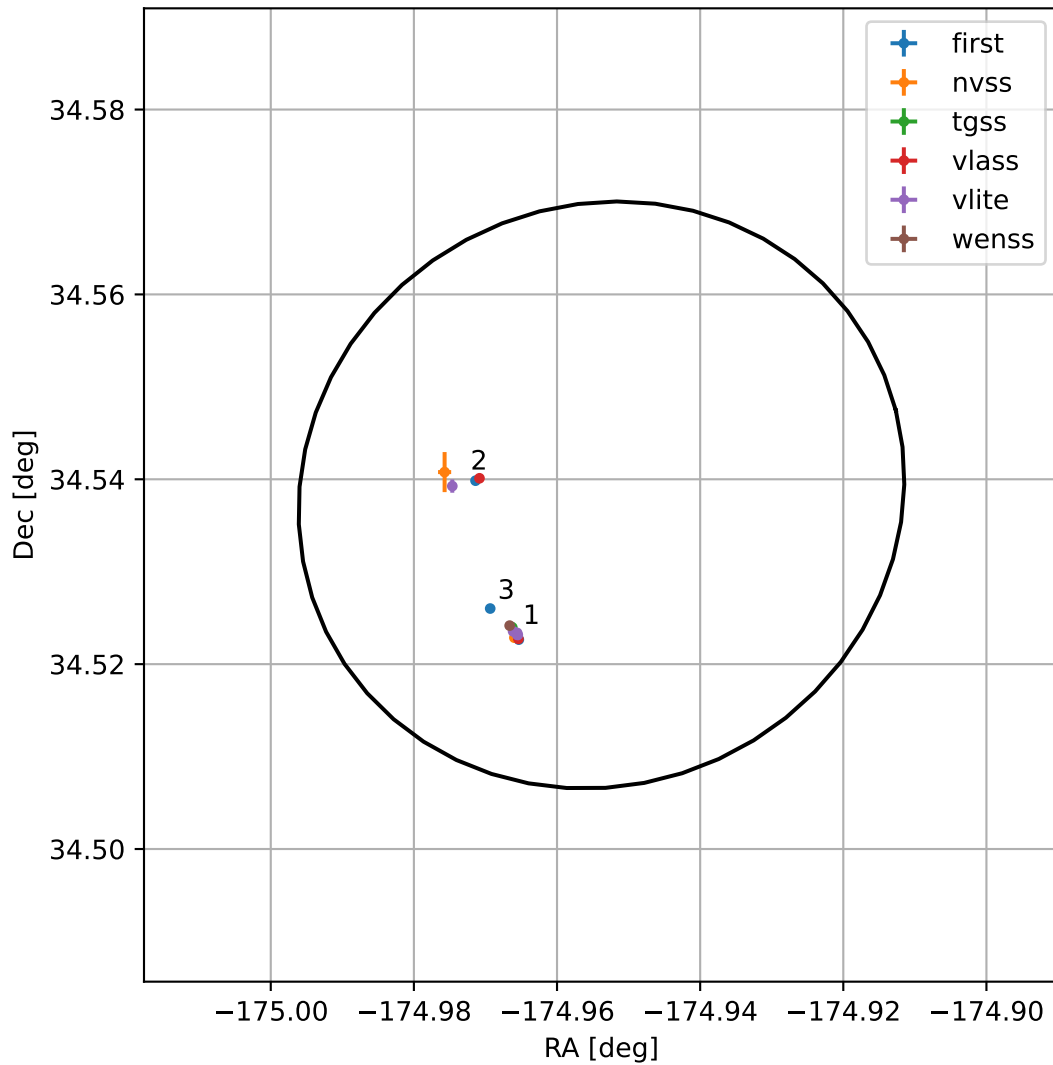
4FGL J1220.1+3432
