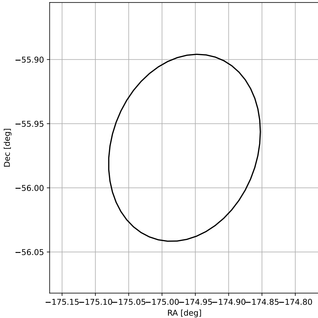
4FGL J1220.1-5558
