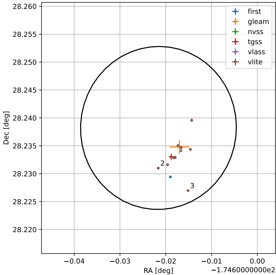
4FGL J1221.5+2814
