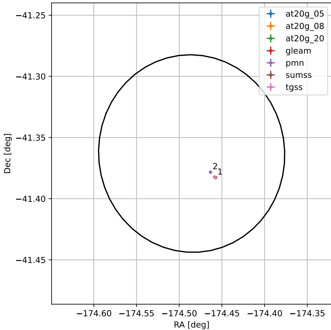
4FGL J1222.0-4121
