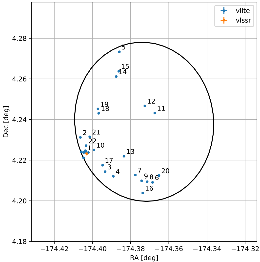
4FGL J1222.5+0414
