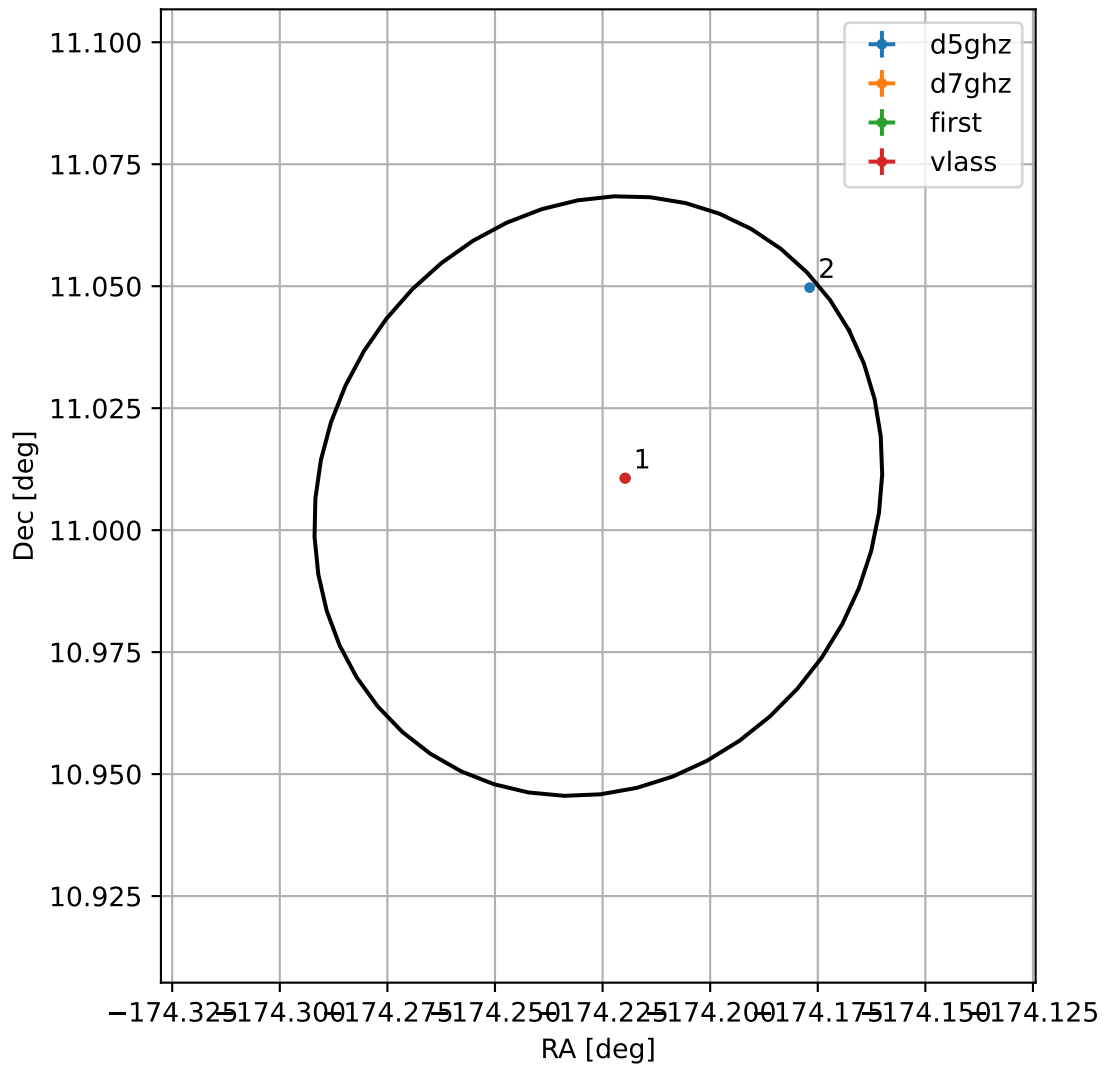
4FGL J1223.0+1100
