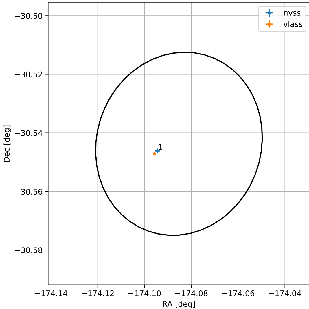
4FGL J1223.6-3032
