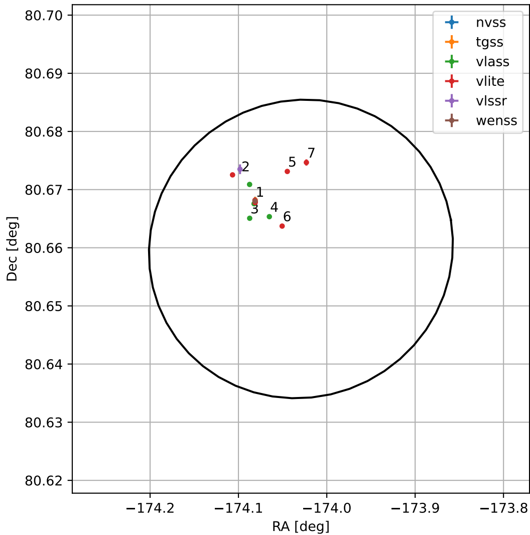
4FGL J1223.8+8039
