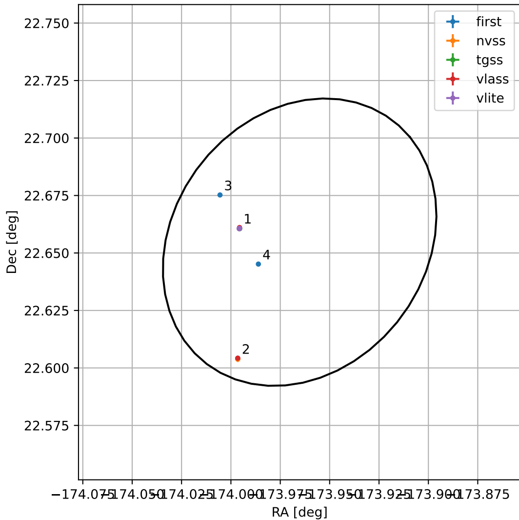
4FGL J1224.1+2239
