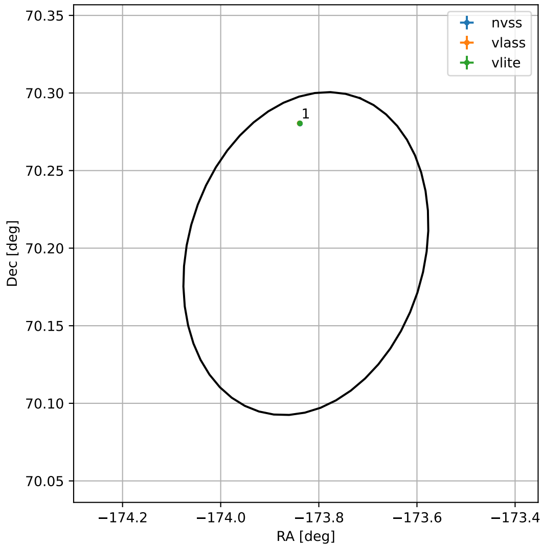
4FGL J1224.6+7011
