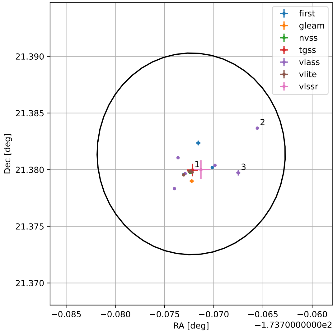
4FGL J1224.9+2122
